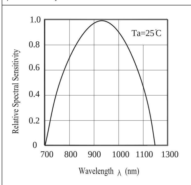
Spectral Sensitivity
